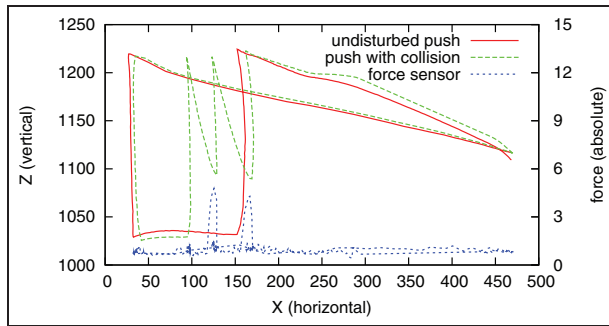
Figure 12. Trajectories of the right hand during two pushes. The trajectory represented by the continuous line was recorded during an undisturbed push, while the dashed one was generated when the hand hit an obstacle twice before it could be lowered besides the object. The forces arising due to collisions with the obstacle are shown by the dotted line.
