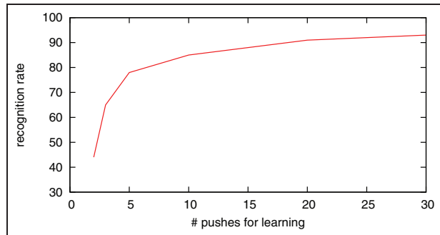
Figure 10. The performance of multiview object recognition with respect to the number of training images acquired from different viewpoints.
