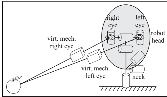
Figure 8. ARMAR-III head kinematics with two translational, virtual degrees of freedom.
