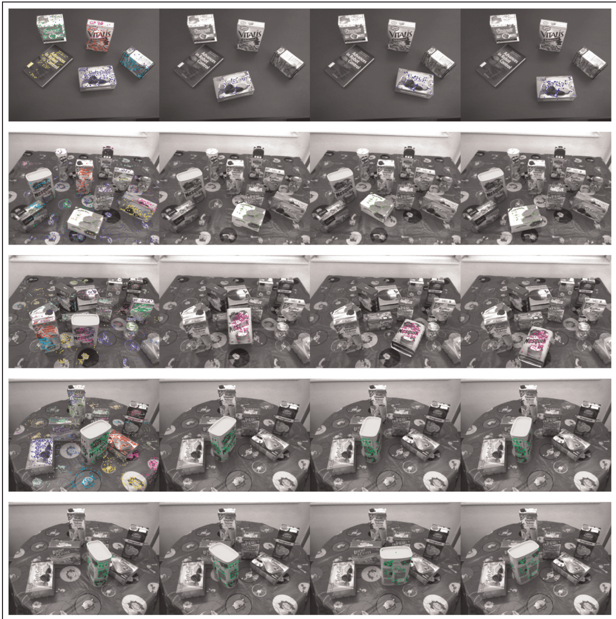
Figure 9. The first three rows show object discovery and segmentation in different settings: in each row, the first image depicts the initial object hypotheses that were generated. As can be seen, their quality decreases in more complex scenes. One hypothesis is then selected for verification and pushed. The second to fourth image in each row show the validated features belonging to that hypothesis after each push. Note that the object is always pushed approximately towards or across a central point in front of the robot, thus staying in the field of view and within the reach of the arms. The last two rows show the segmentation of an object throughout multiple pushes, during which its different sides become visible. This allows the accumulation of object descriptors from multiple viewpoints. Owing to the rather uncontrolled object motion, it may take many pushes until all sides of the object have been revealed. These pictures are an excerpt from a series of 20 pushes.
