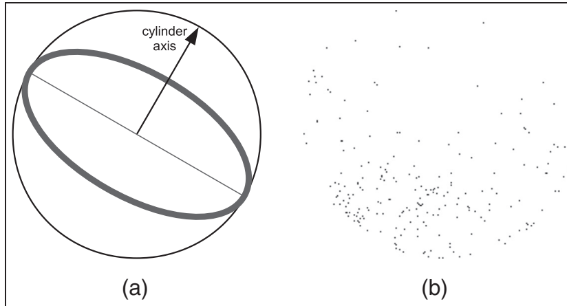
Figure 11. (a) Depiction of how the Gaussian image of a perfect cylinder would look. (b) The Gaussian image resulting from a set of three-dimensional points in a scene containing a cylindrical object on an empty table. Of course only the front side of the object is visible for the cameras, therefore only half of the great circle is contained in the Gaussian image.
