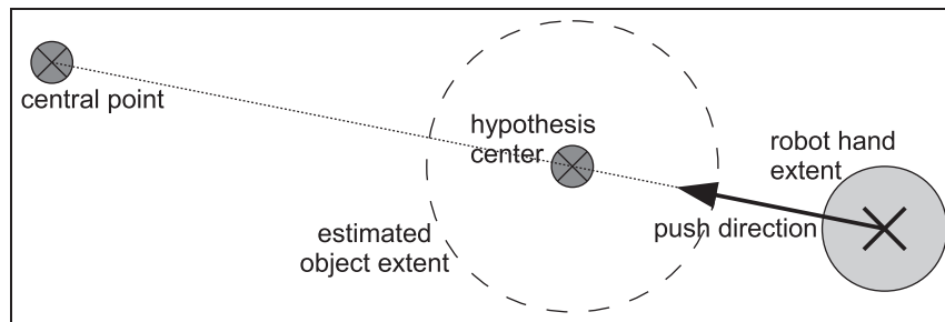
Figure 6. The pushing motion is determined based on the estimated object position and size. The push is always directed towards a fixed central point in front of the robot so that the object stays within its reach and field of view.
