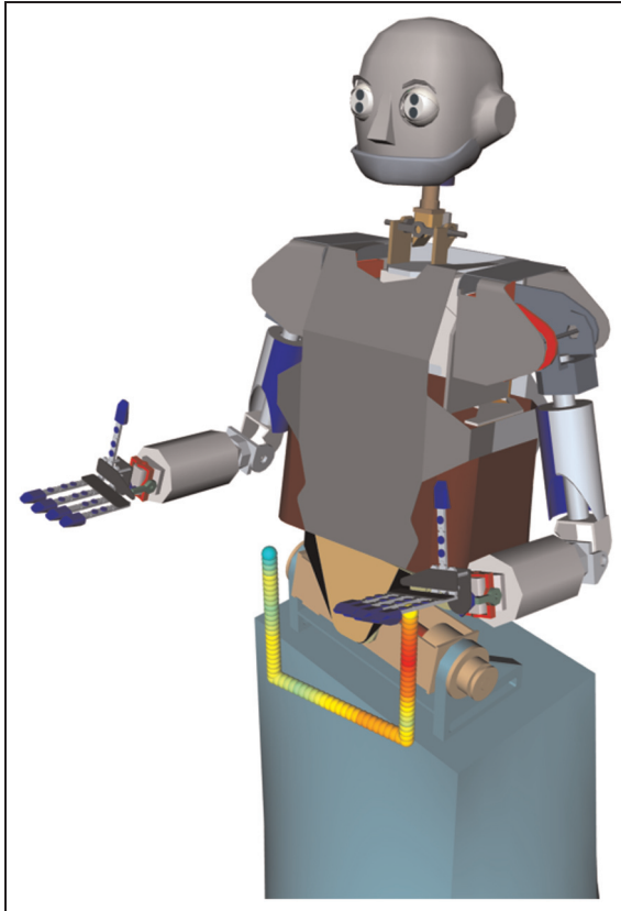
Figure 5. Reachability values on a pushing path for the left hand of ARMAR-III. Dark red dots indicate low, bright yellow dots high reachability values.
